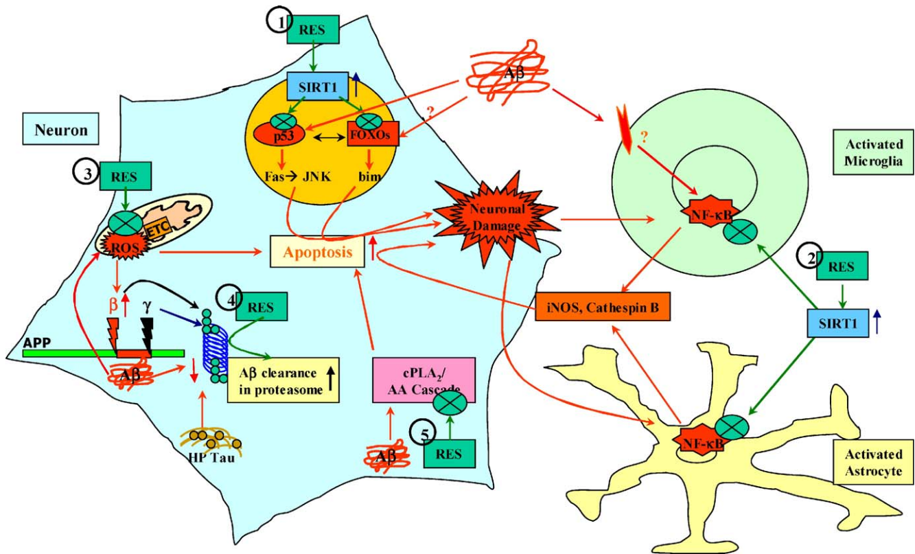
Fig. 1 – Molecular mechanisms of neuronal protection by resveratrol in Alzheimer's disease. (1) Resveratrol-induced SIRT1 deacetylates and represses p53 activity promoted by A \beta in neurons and prevent apoptotic death in these neurons. In addition, SIRT1 suppresses apoptotic activities of FOXO proteins and promotes neuronal survival. (2) Resveratrol-induced SIRT1 inhibits nuclear factor kappa B and subsequently suppresses nitric oxide synthase (iNOS) and cathepsin B, the two toxic factors that mediate neurodegeneration in microglia and astrocytes, and protects AD neurons against A \beta -induced toxicity. (3) Resveratrol functions as an antioxidant and possibly prevents reactive oxygen species-induced A \beta production and apoptosis-mediated neurodegeneration. (4) Resveratrol modulates the ubiquitin proteasome system via an unknown mechanism and promotes hastened A \beta degradation without affecting A \beta -producing metabolism. (5) Resveratrol blocks nitric oxide-induced phospholipase A _2 /arachidonic acid cascades in the cytoplasm and prevents apoptotic death of neurons.
